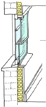
EXISTING FABRIC UPGRADE - Secondary vacuum glazing - Internal wall insulation
