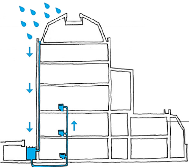
RAINWATER HARVESTING FOR TOILET FLUSHING
