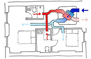
WHOLE HOUSE VENTILATION WITH HEAT RECOVERY
