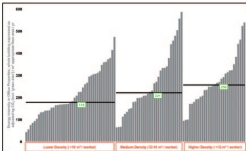
Fig 3: BBP office carbon benchmarking – carbon per floor area indicator (kgCO 2 /m 2 /year), categorised into three bands of worker density (m 2 /worker).
