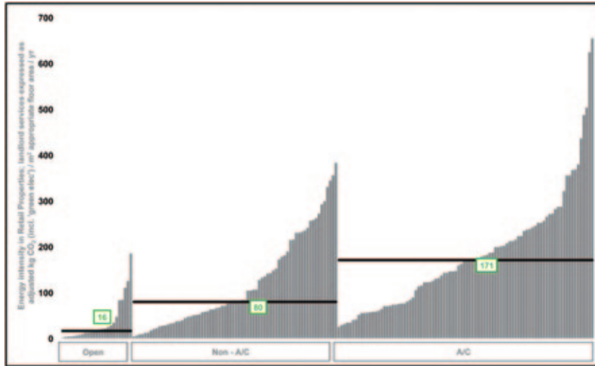
Fig 1: BBP retail carbon benchmarking - carbon per floor area indicator (kgCO 2 /m 2 /year), categorised into three bands based on type of HVAC system (OSCAR).
