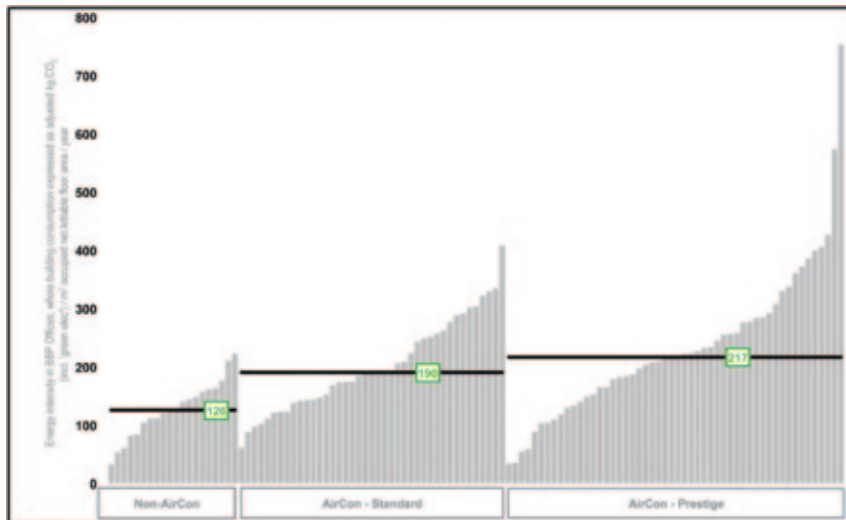
Fig 2: BBP office carbon benchmarking - carbon per floor area indicator (kgCO 2 /m 2 /year), categorised into three bands based on type of HVAC system (ECON 19).
